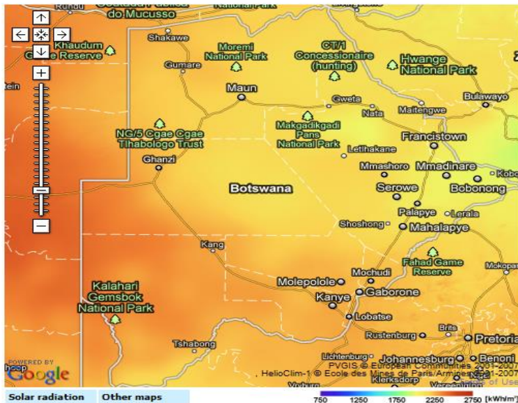
Figure 6: Detailed solar hotspots of global irradiation \text{KWh/m}^2/\text{year} for Botswana
